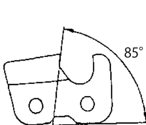
Side blade 85°
