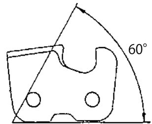
Upper cutting blade 60°
